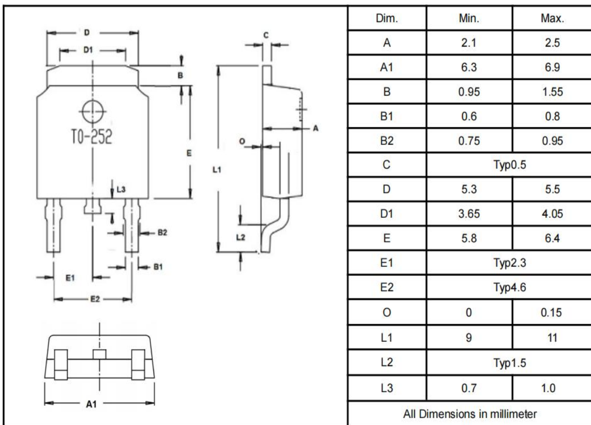
TO-252
