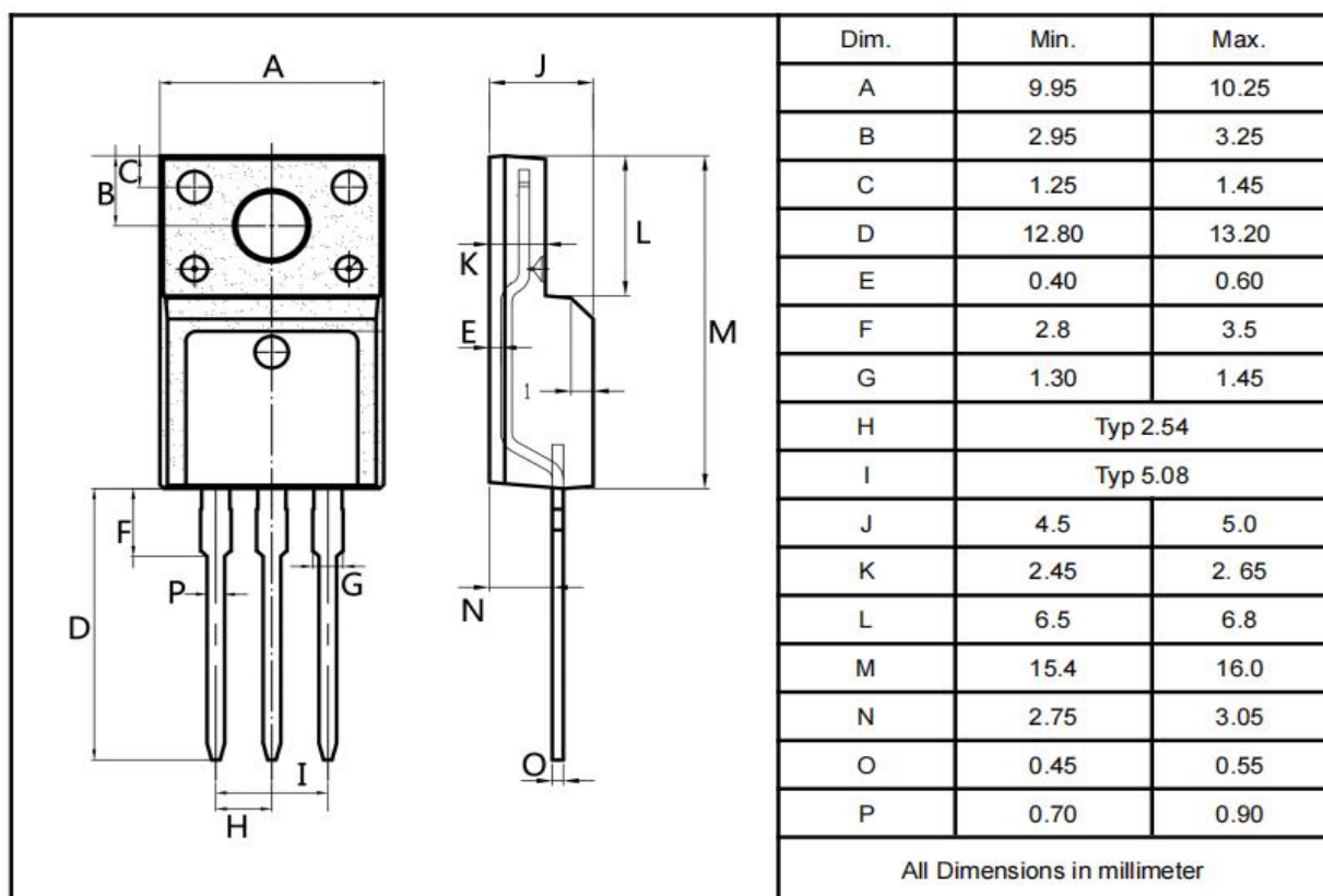
TO-220F
