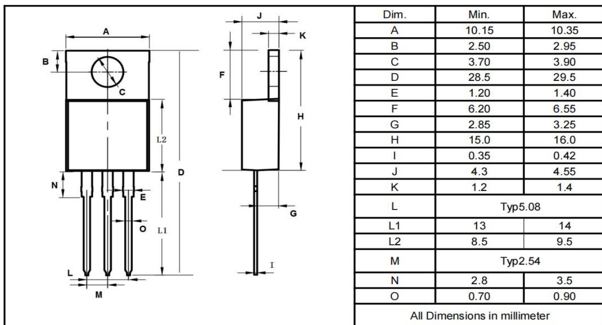
TO-220AB
